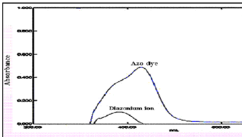
Figure 3.5: Absorbance Spectrum of Diazonium Ion and Azo Dye using MSP-EAA
