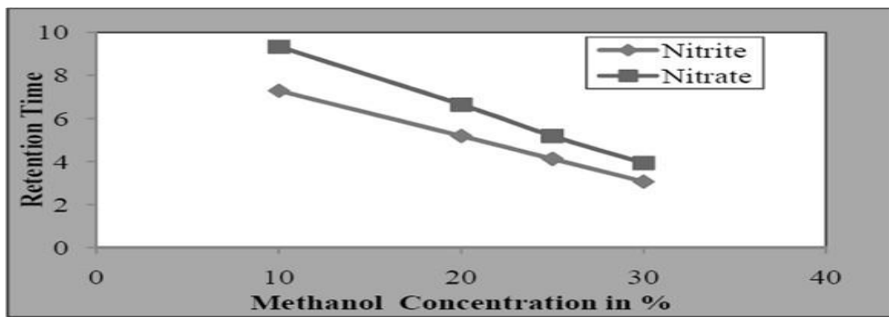
Figure 3.1: Effect of Methanol concentration variation in the mobile phase
