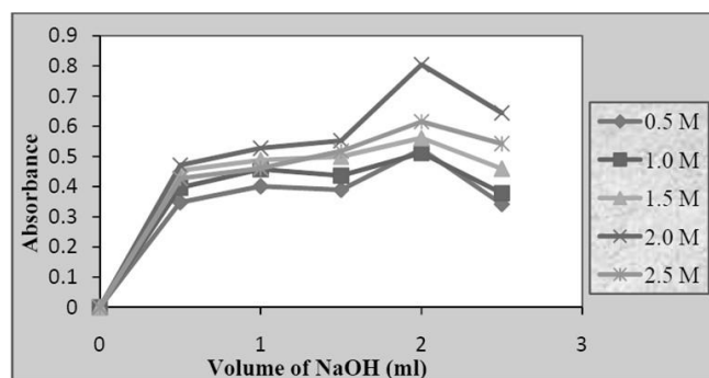
Figure 4.4: Absorbance Variation for MSP Reagent of varying concentration and NaOH volume
