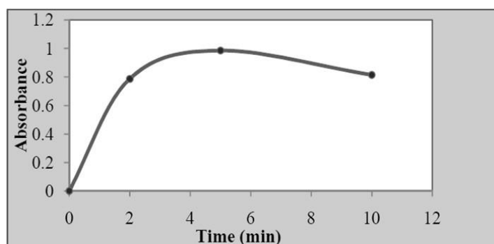
Figure 4.5: Absorbance Variation with Varying Time of Diazotization for MSP
