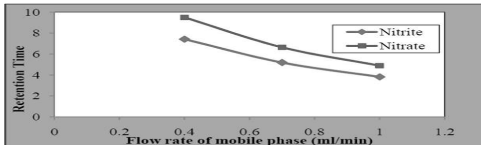
Figure 3.3: Effect of Mobile Phase Flow Rate Variation
