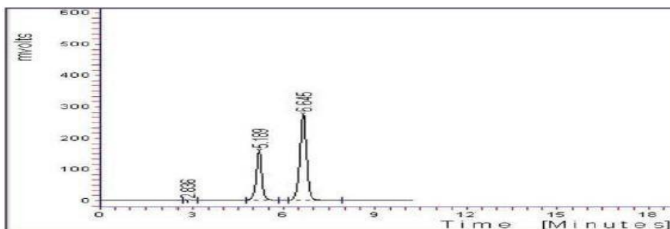
Figure 3.4: Zinc nitrite and nitrate separation in selected mobile phase, showing retention time for nitrite (1ppm) and nitrate (10ppm)
