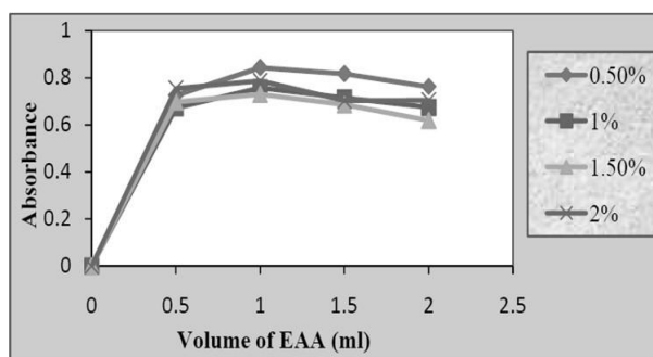
Figure 4.1: Absorbance Variation with varying Attentioness and MSP EAA solutions volume
