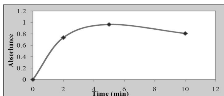
Figure 4.6: Absorbance Variation with Varying Time of Diazotization for MTCP
