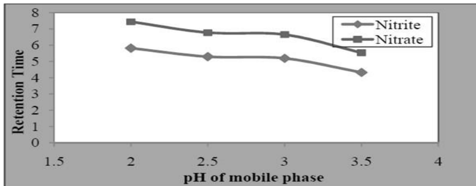
Figure 3.2: Effect of mobile-phase pH variations
