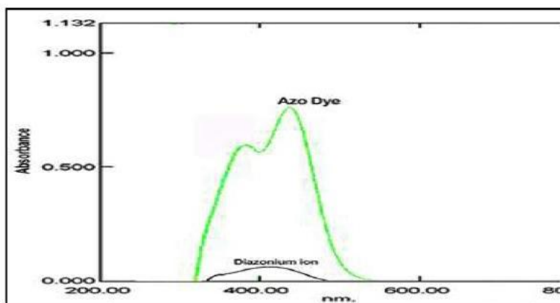
Figure 3.6: Absorbance Spectrum of Azo Dye and Diazonium Ion using MTCP-EAA
