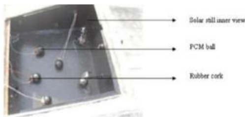
Figure 7. Single slope solar still with phase change material (inside view) [23]
