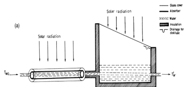
Figure 3. Single slope solar still integrated with tubular solar collector [16]
