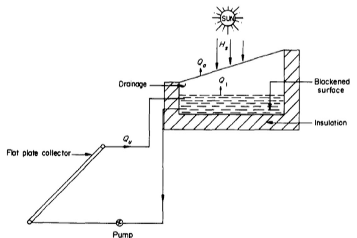
Figure 2. Single slope solar still coupled to flat plate collector [12]
