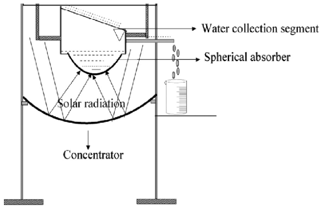
Figure 6. Schematic diagram of hemispherical absorber concentrator assisted solar still [22]
