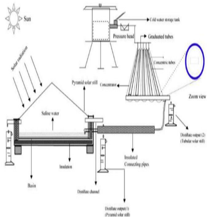
Figure 9. Schematic view CPC-CTSS with pyramid solar still [24]
