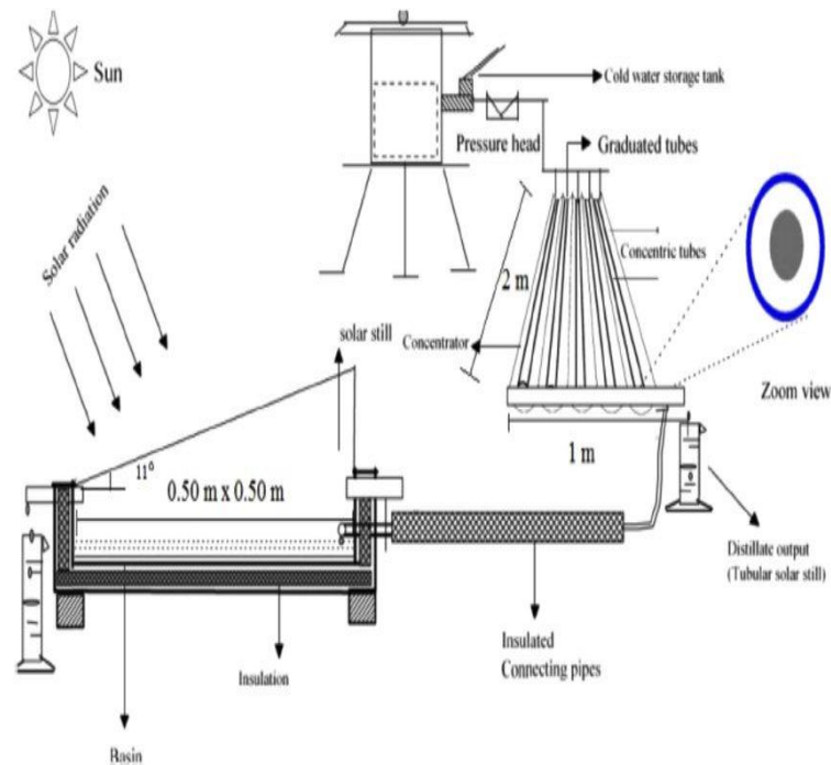
Figure 8. Schematic view of CPC-CTSS coupled with single slope solar still
