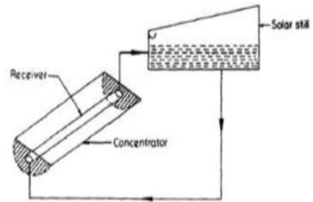
Figure 5. Schematic diagram single basin solar still with parabolic trough collector [19]
