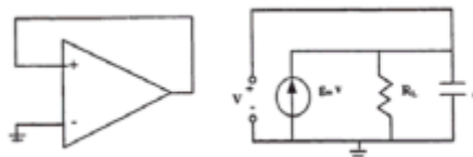
Fig. 8 The small signal model
