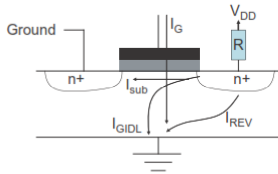
Figure 2. Sources of Transistor Leakage Table 1. Main Sources of Transistor Leakage
