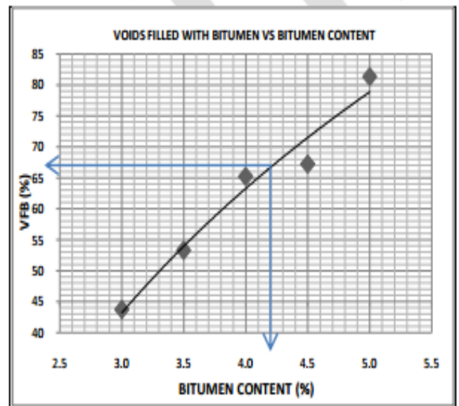
Figure 1:- Voids Filled with Bitumen V/s. Bitumen Content
