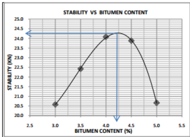
Figure 2:- Stability V/s. Bitumen Content
