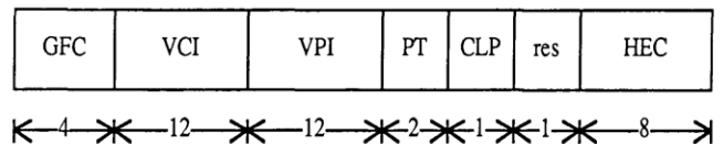
Figure 2: The cell-header format for the U.N.I.; dimensions in bits.
