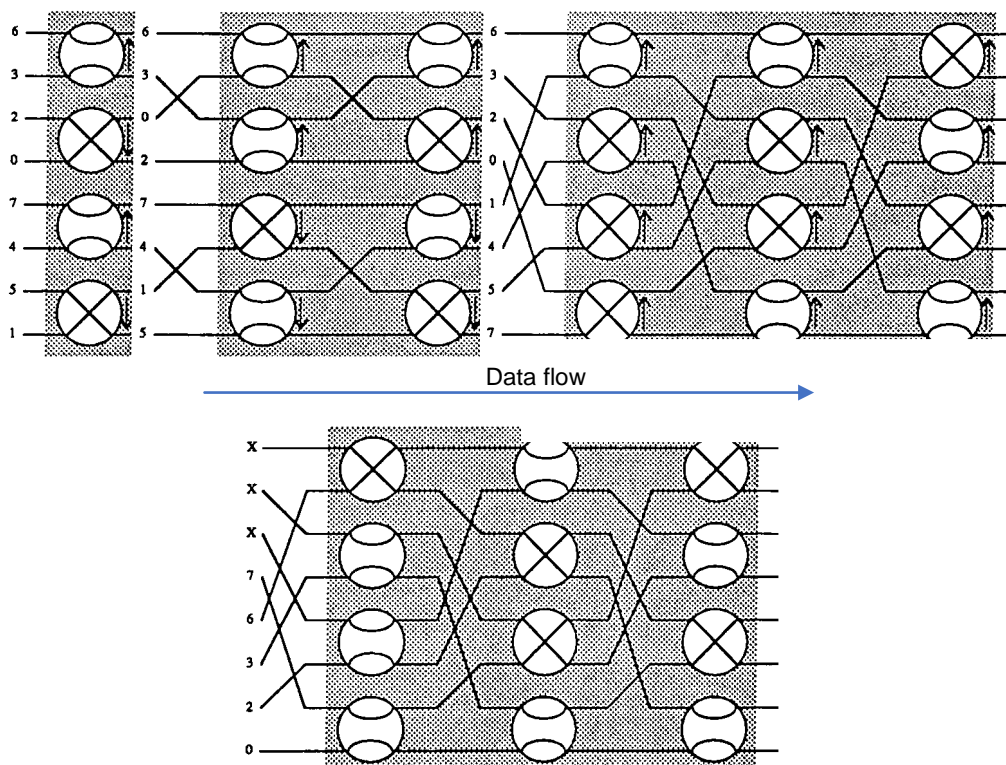
Figure 5: Connexion graphs for the two main phases of a Starlite switch. The top graph performs the perfect shuffle to sort the inputs into order (the arrows point to the output that should have the larger of the two inputs); the lower graph is the expansion phase that uses the bit fields of the output port to determine the route.
