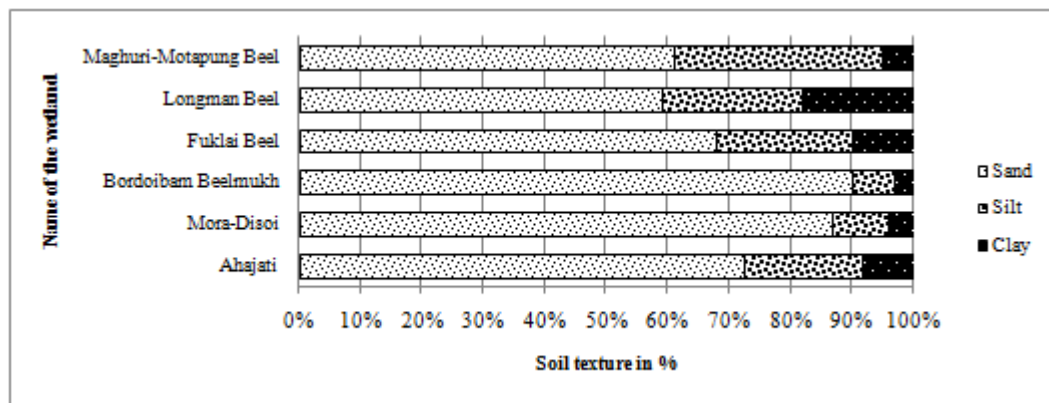
Fig.3. Percentage of different soil texture (includes Sand, Silt and clay) in selected wetlands
