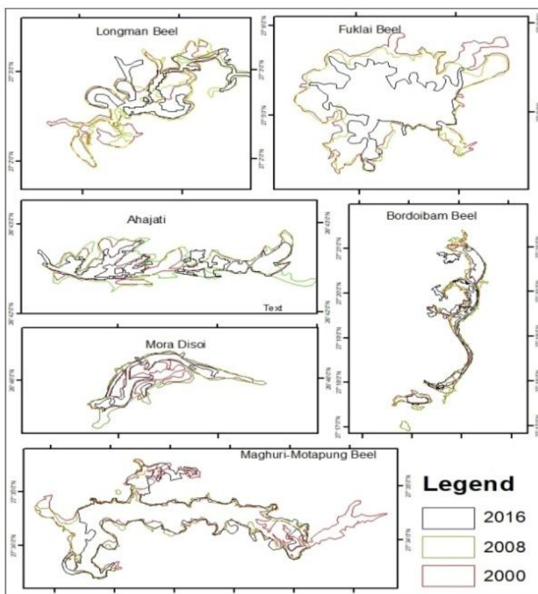
Fig.2: Map of wetland area changes from 2000 to 2008 and 2017
