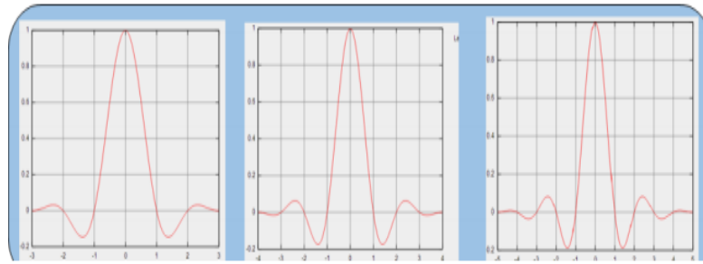
Fig.2.Sinc interpolation functions of orders 3, 4 and 5
