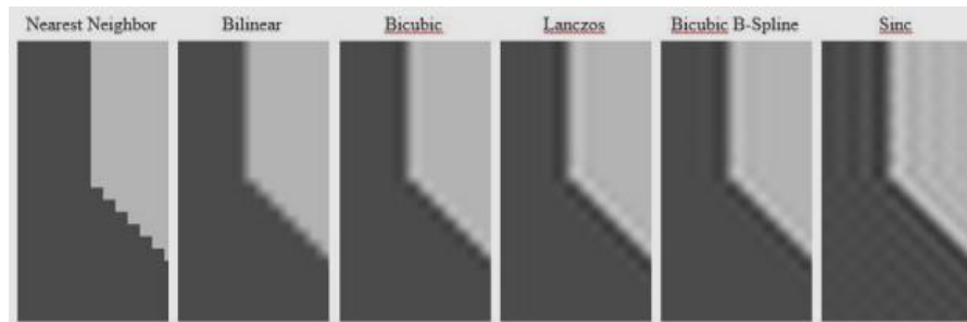
Fig.3.Linear interpolation of a step edge: a balance between staircase artifacts and ripples [12].
